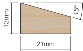
▲ LG1320 For unrebated screen frames.
