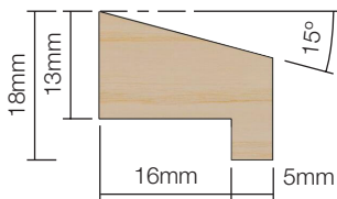
▲ LG1321 For 44mm thick doors or rebated screen frames.
